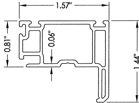
4 TOP & BOTTOM RAIL
