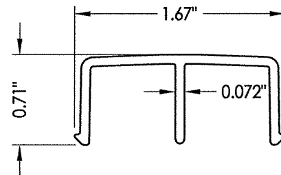
16 ROLLER TRACK
