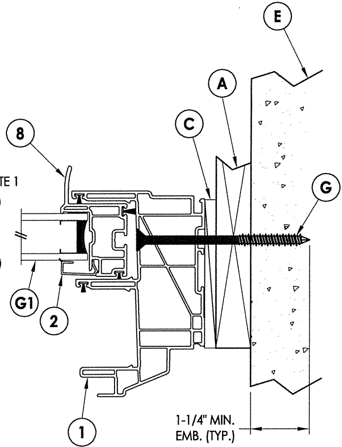
2/2 HORIZONTAL CROSS SECTION 1X Buck Masonry Construction
