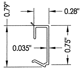
2 GLAZING BEAD
