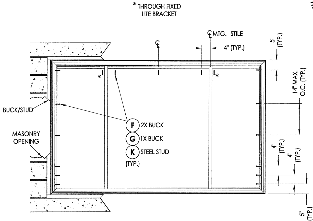
FRAME ANCHORING
