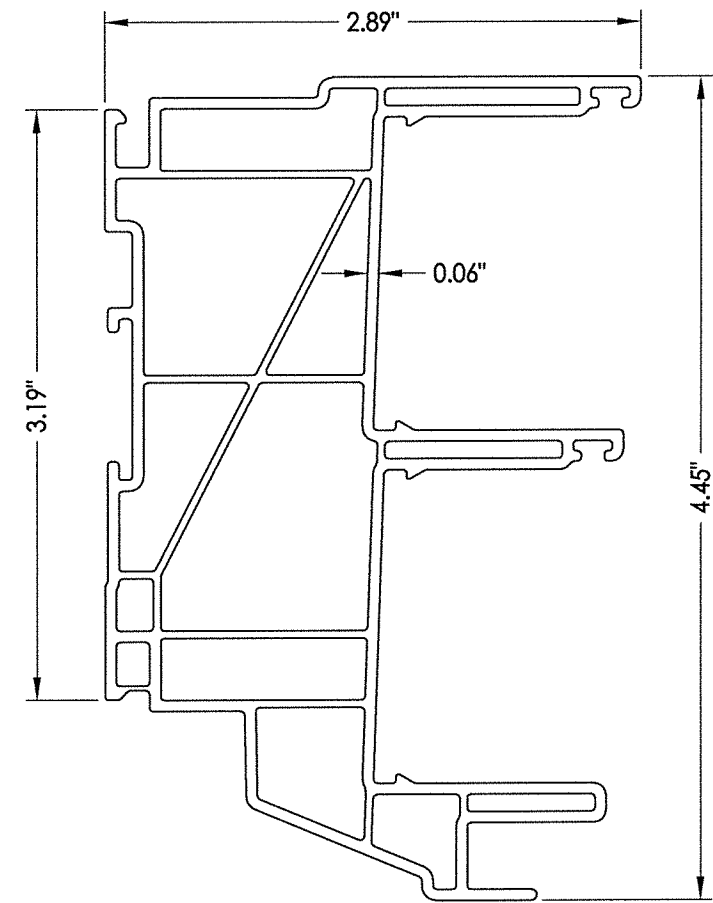
1 FRAME
