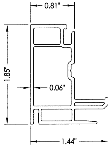
6 MEETING STILE
