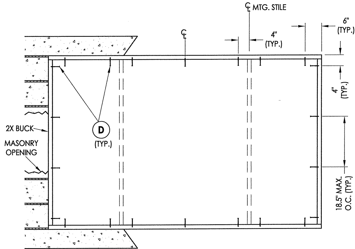
2X BUCK ANCHORING
